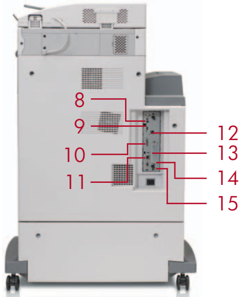
HP Color LaserJet 4730x mfp rear view
